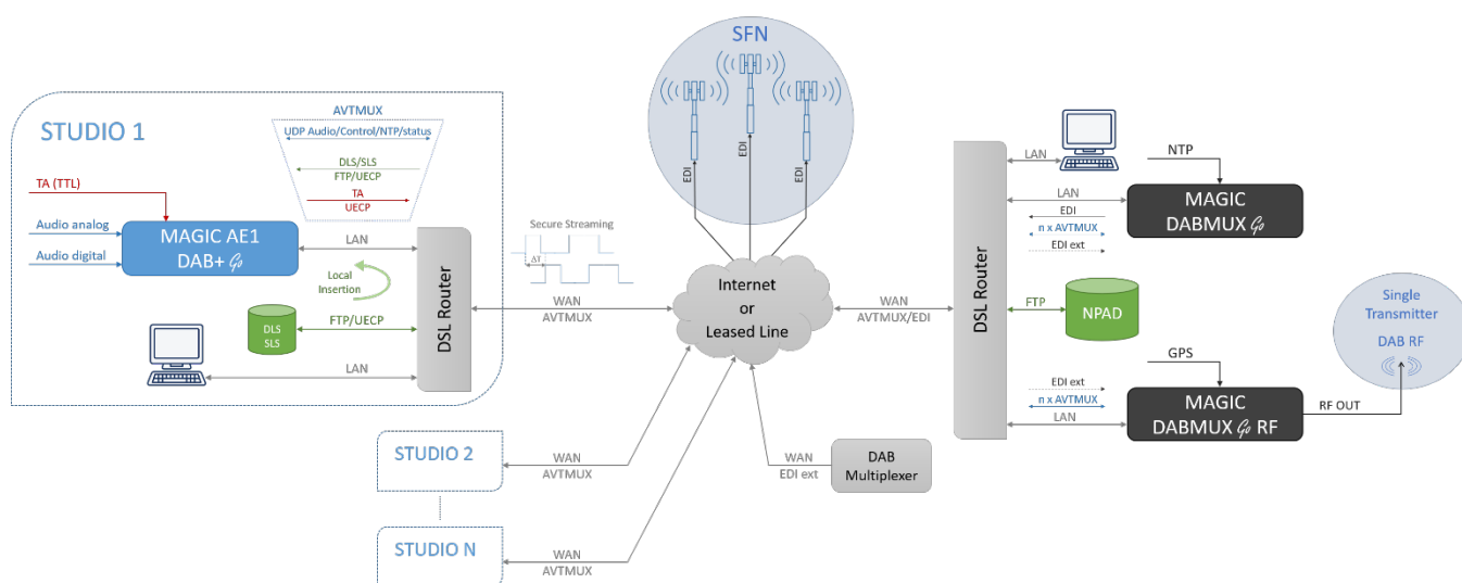
Small Scale DAB headend
